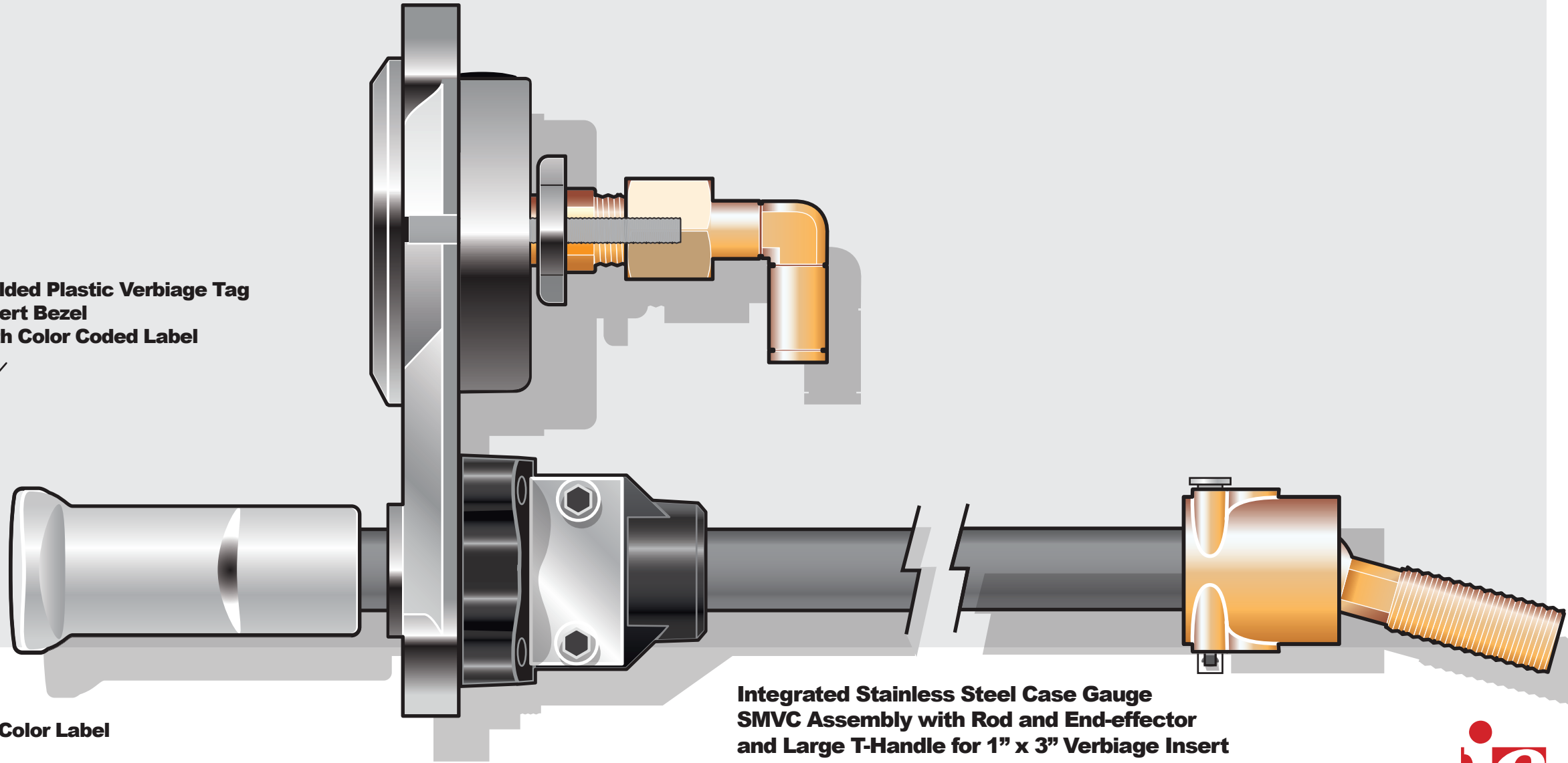
SMVC Assembly with Rod and End-effector (various rod lengths available) and Large T-Handle for 1" x 3" Verbiage Insert
